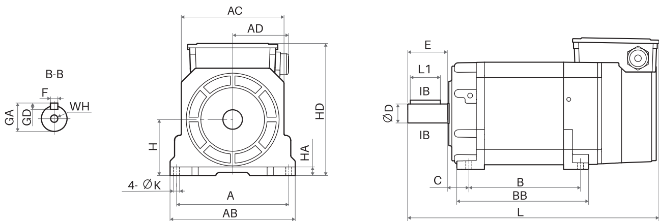
Z18PB Z18PC Z18PE-Z18PH 机座
