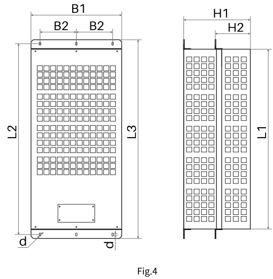
Resistance Box Overall and Mounting Dimensions
