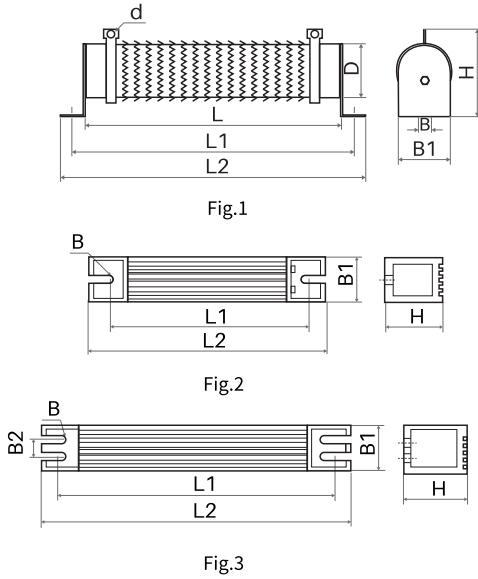
Brake Resistor Overall and Mounting Dimensions
